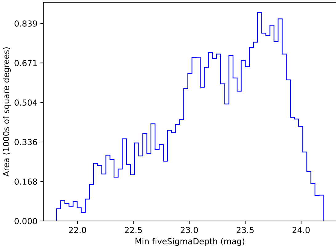
too_elab_r16_d3_giz_v3.4_10yrs Yr 1 r band: Min fiveSigmaDepth
