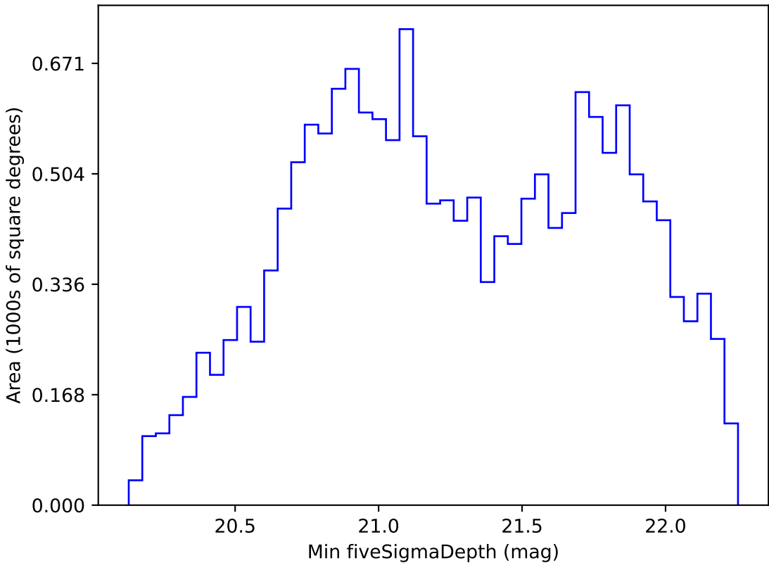
too_elab_r16_d3_giz_v3.4_10yrs WFD z band: Min fiveSigmaDepth
