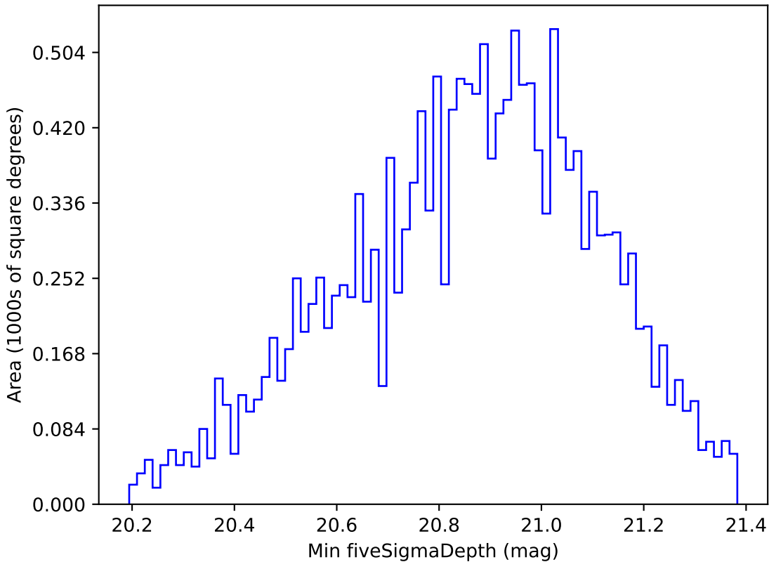
too_elab_r16_d3_giz_v3.4_10yrs WFD y band: Min fiveSigmaDepth
