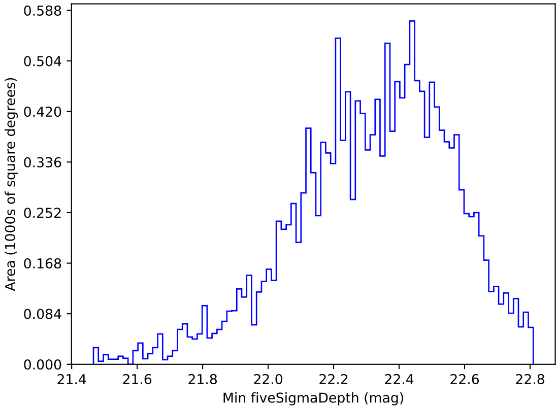
too_elab_r16_d3_giz_v3.4_10yrs WFD u band: Min fiveSigmaDepth
