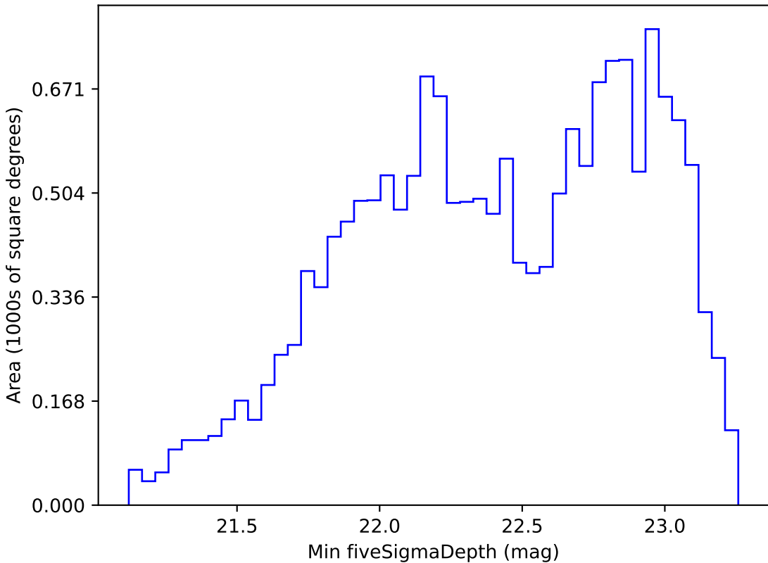
too_elab_r16_d3_giz_v3.4_10yrs WFD r band: Min fiveSigmaDepth
