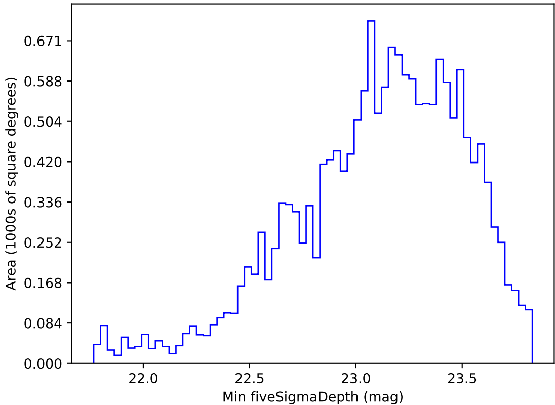
too_elab_r16_d3_giz_v3.4_10yrs WFD g band: Min fiveSigmaDepth
