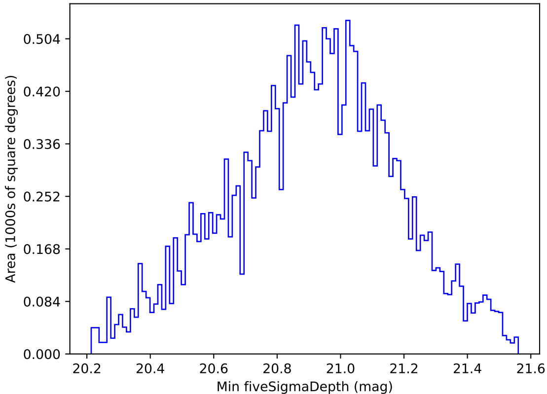
too_elab_r16_d3_giz_v3.4_10yrs All sky y band: Min fiveSigmaDepth
