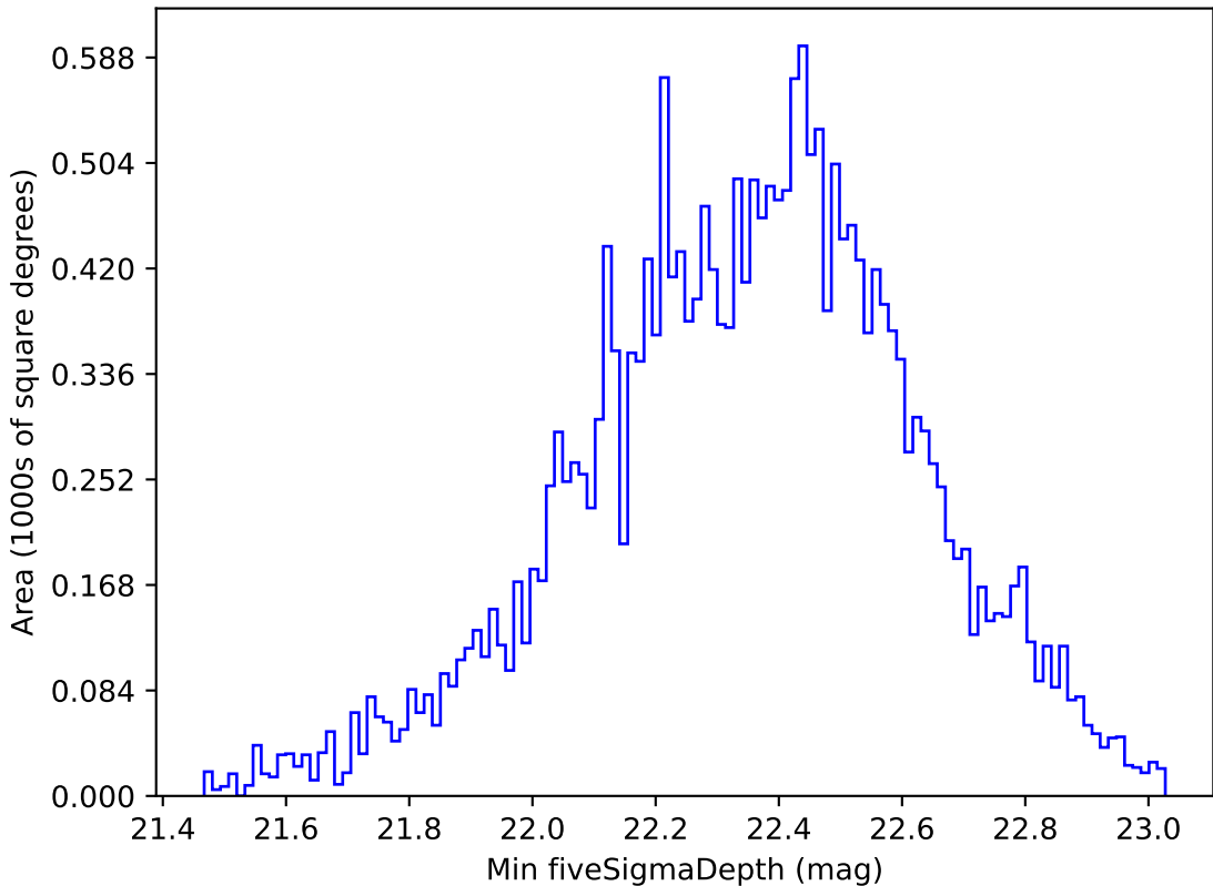
too_elab_r16_d3_giz_v3.4_10yrs All sky u band: Min fiveSigmaDepth
