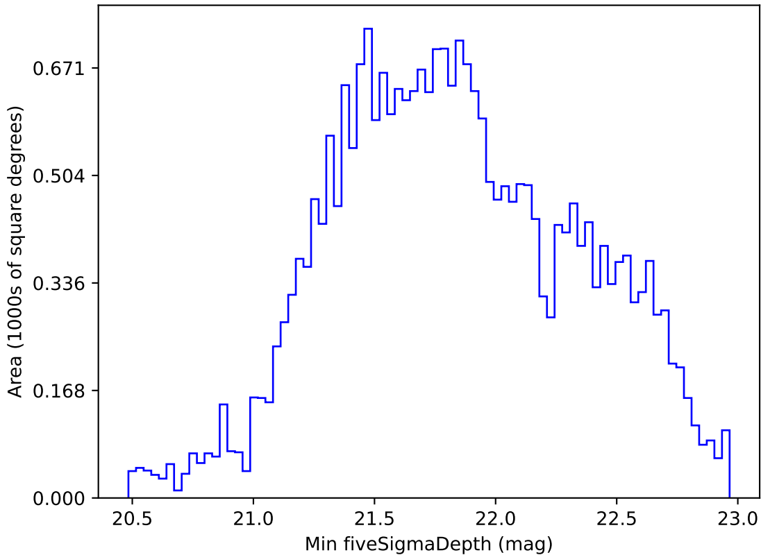
too_elab_r16_d3_giz_v3.4_10yrs All sky i band: Min fiveSigmaDepth
