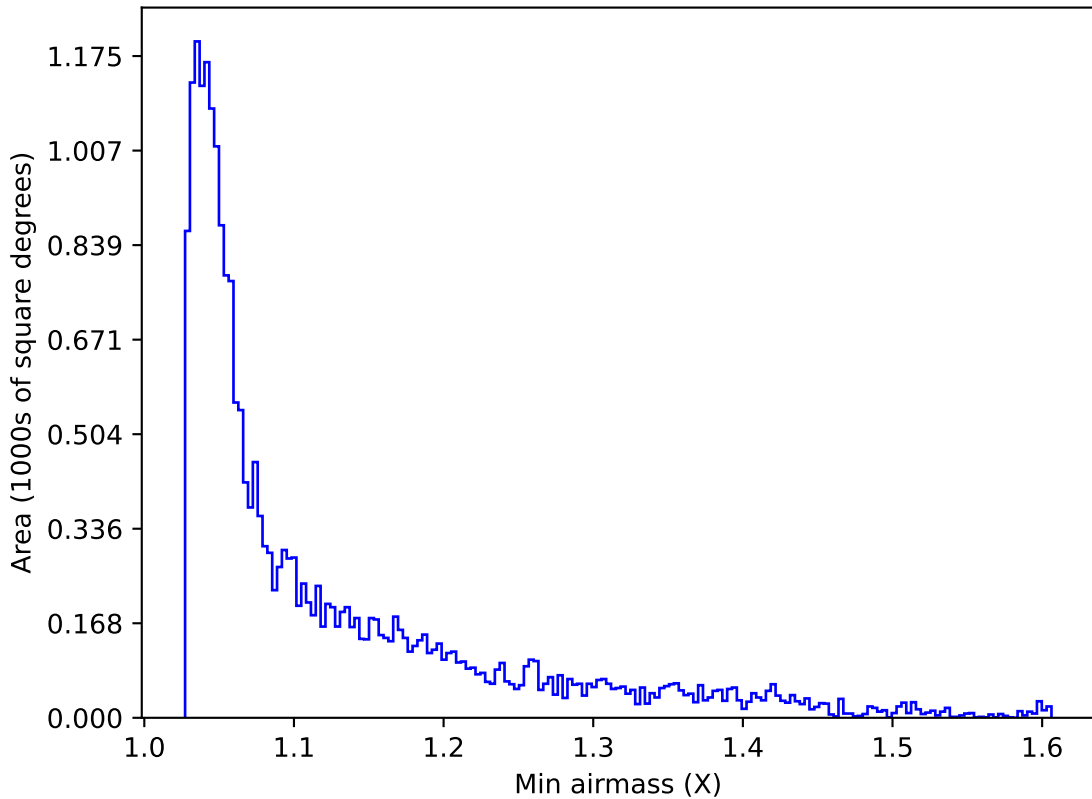
too_elab_r16_d3_giz_v3.4_10yrs Yr 1 y band: Min airmass
