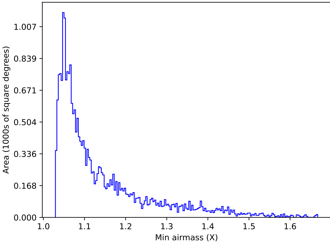
too_elab_r16_d3_giz_v3.4_10yrs Yr 1 u band: Min airmass
