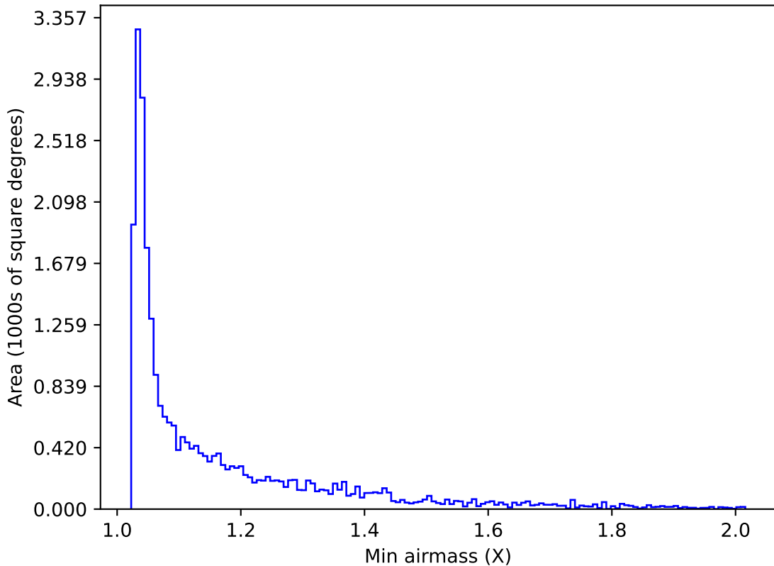
too_elab_r16_d3_giz_v3.4_10yrs Yr 1 i band: Min airmass
