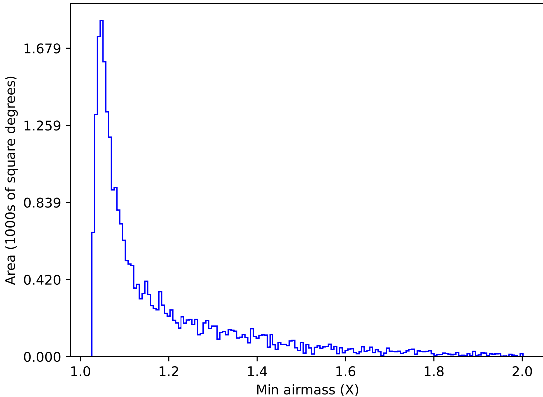
too_elab_r16_d3_giz_v3.4_10yrs Yr 1 g band: Min airmass
