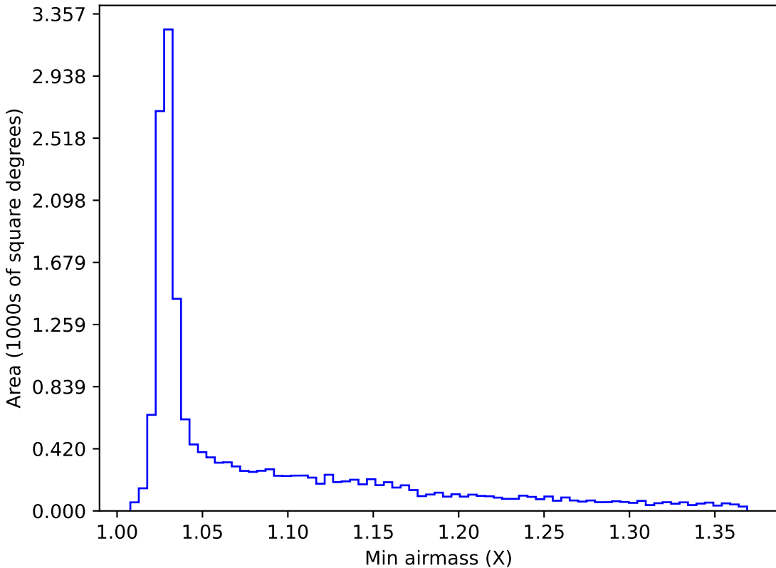
too_elab_r16_d3_giz_v3.4_10yrs WFD z band: Min airmass
