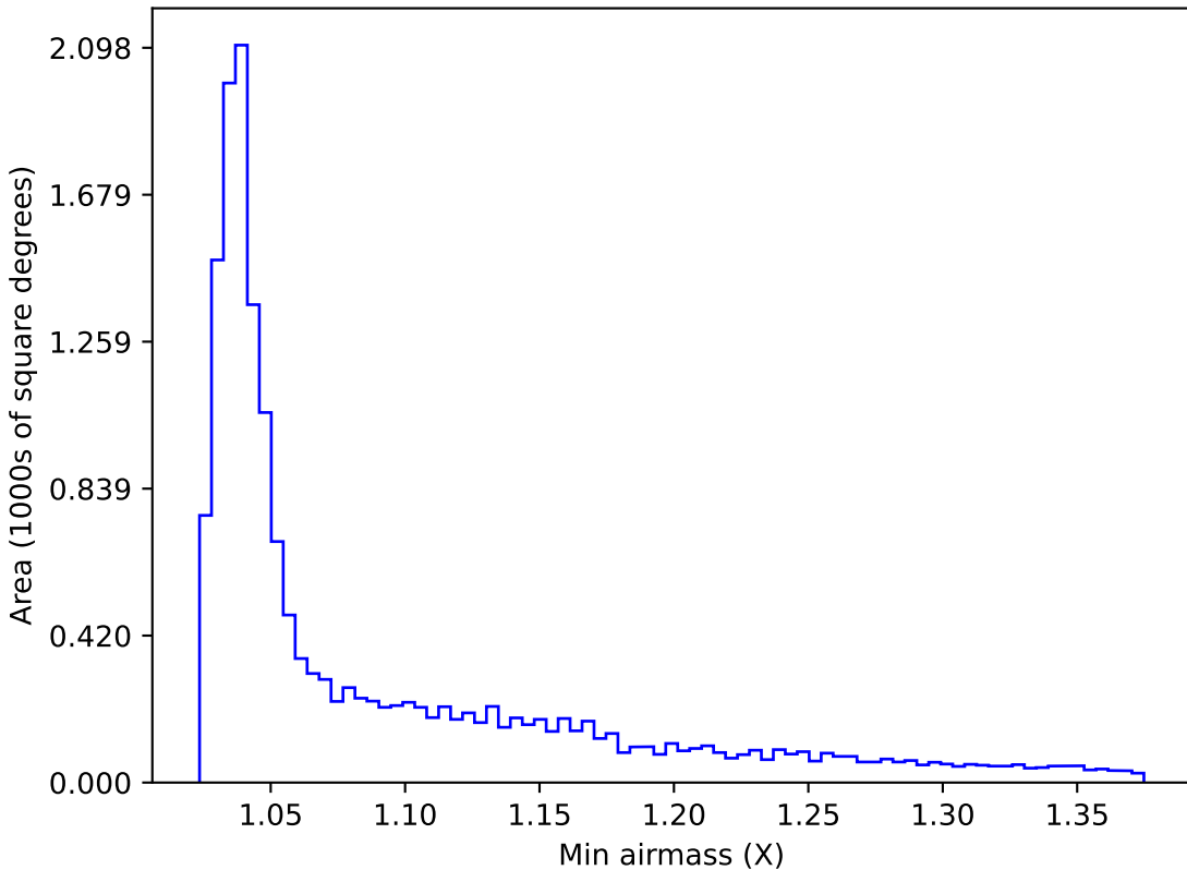
too_elab_r16_d3_giz_v3.4_10yrs WFD u band: Min airmass
