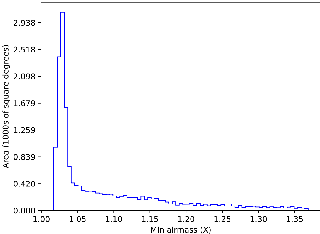
too_elab_r16_d3_giz_v3.4_10yrs WFD r band: Min airmass
