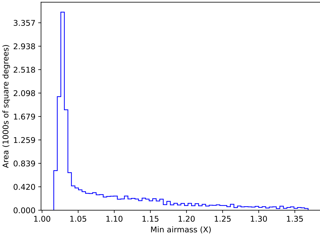
too_elab_r16_d3_giz_v3.4_10yrs WFD i band: Min airmass
