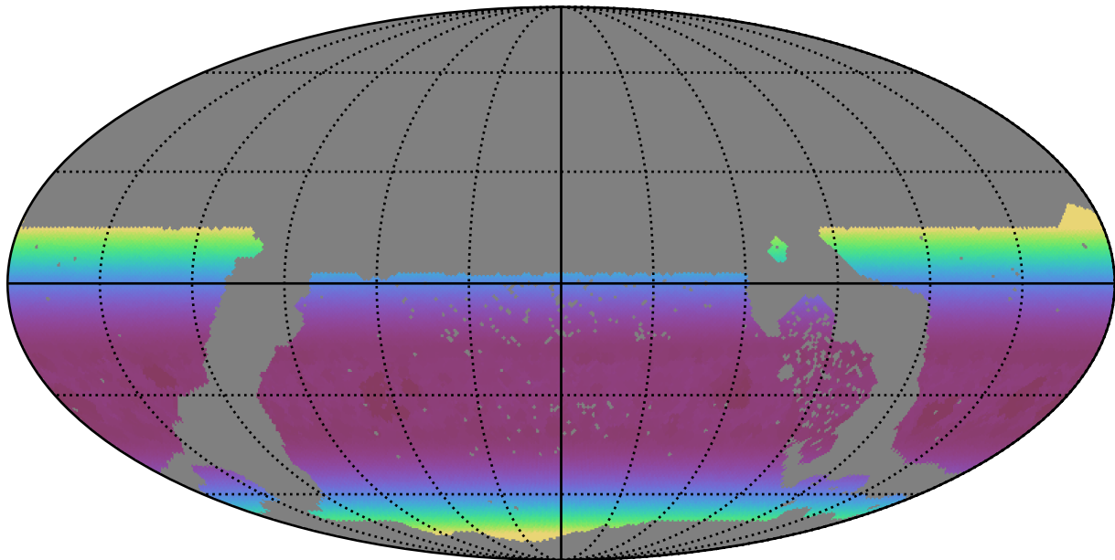
too_elab_r16_d3_giz_v3.4_10yrs WFD all bands: Min airmass
