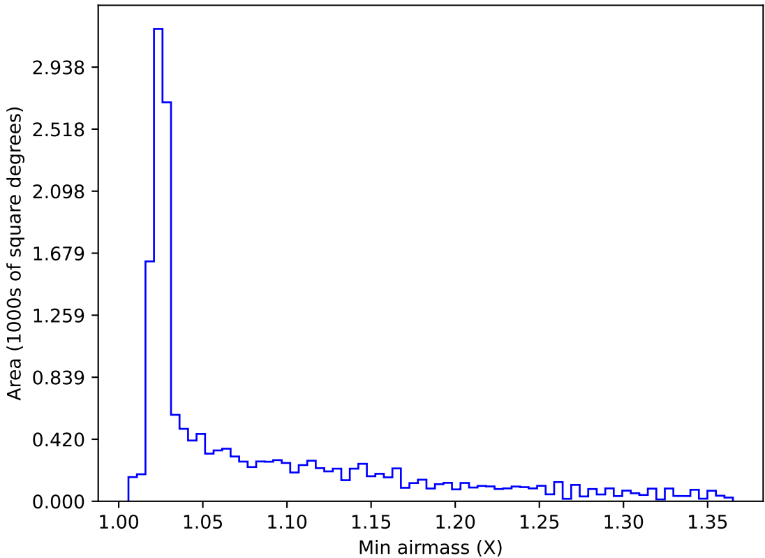
too_elab_r16_d3_giz_v3.4_10yrs WFD all bands: Min airmass
