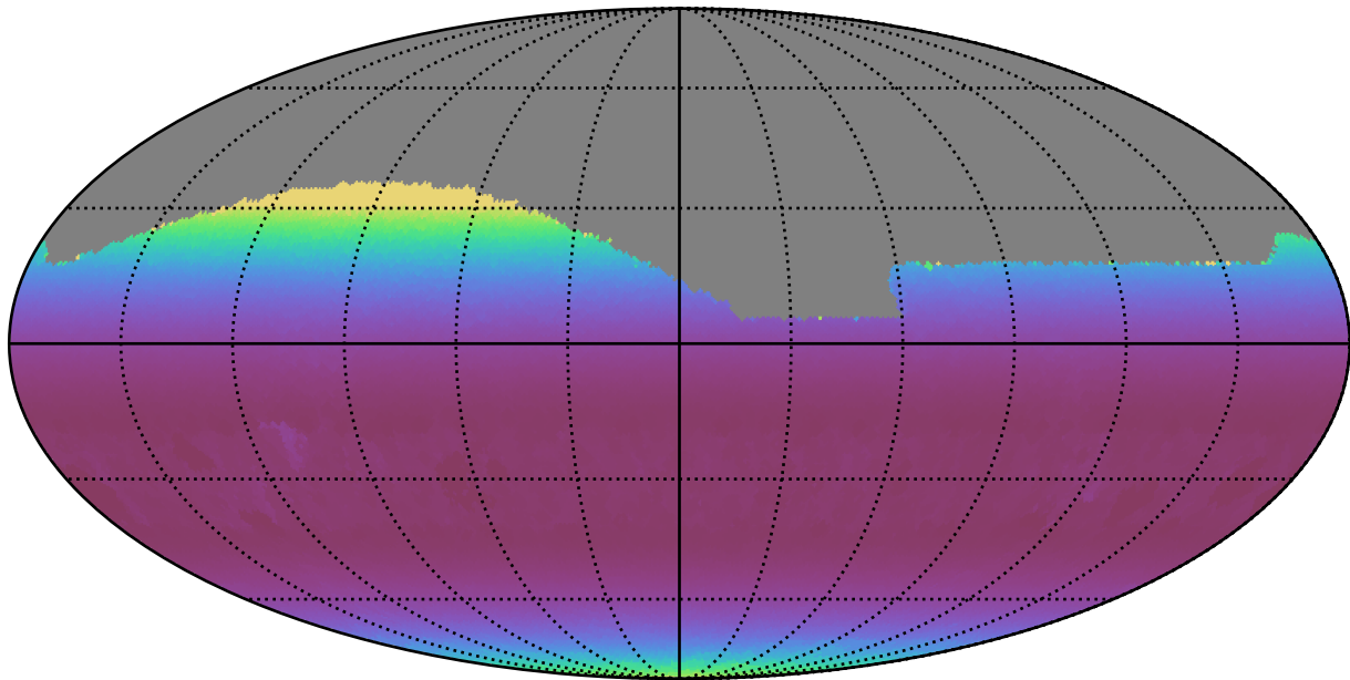
too_elab_r16_d3_giz_v3.4_10yrs All sky g band: Min airmass
