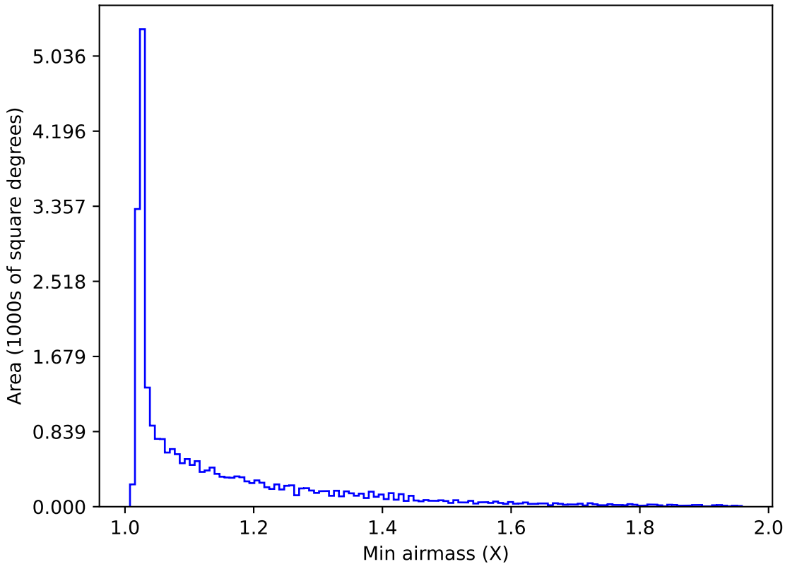
too_elab_r16_d3_giz_v3.4_10yrs All sky all bands: Min airmass
