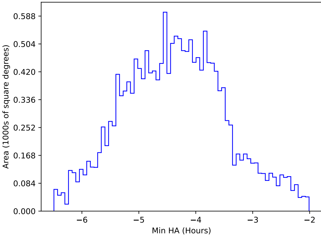
too_elab_r16_d3_giz_v3.4_10yrs WFD z band: Min HA
