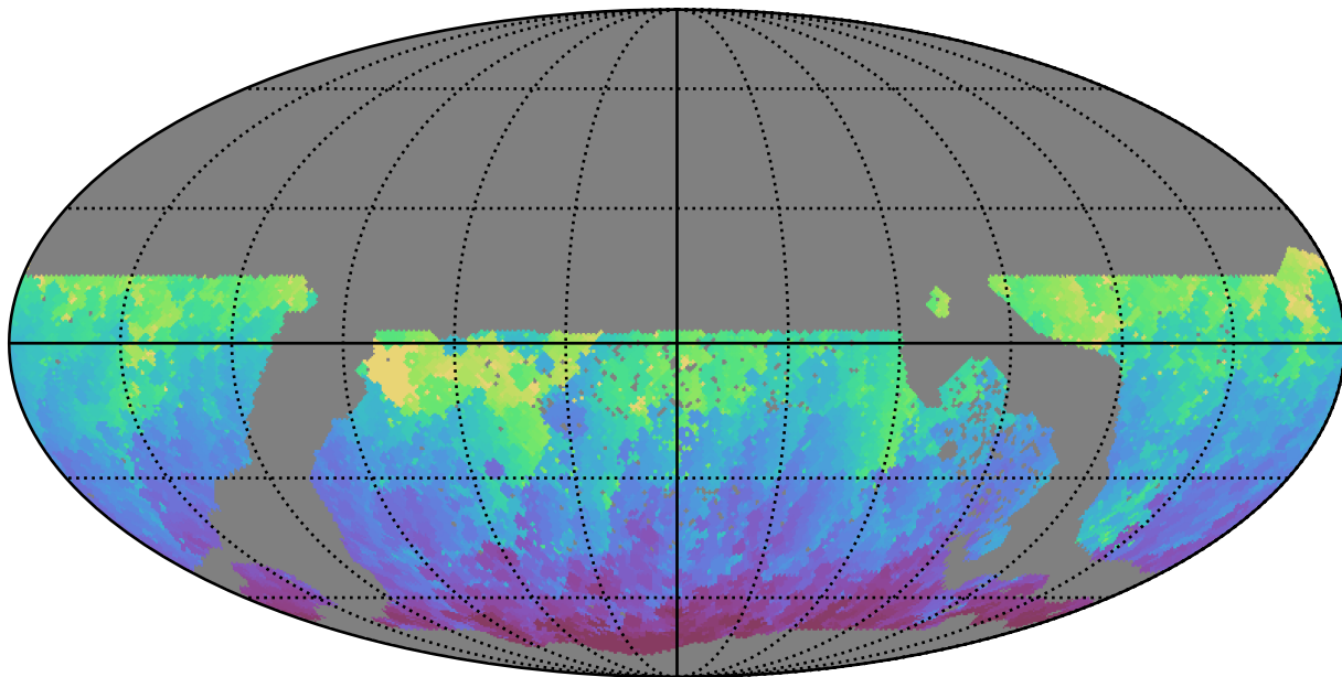
too_elab_r16_d3_giz_v3.4_10yrs WFD g band: Min HA
