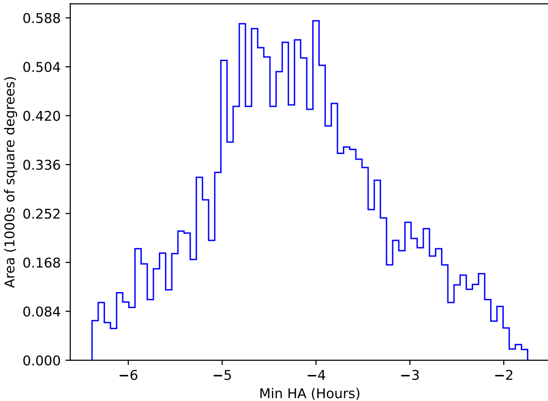
too_elab_r16_d3_giz_v3.4_10yrs WFD g band: Min HA
