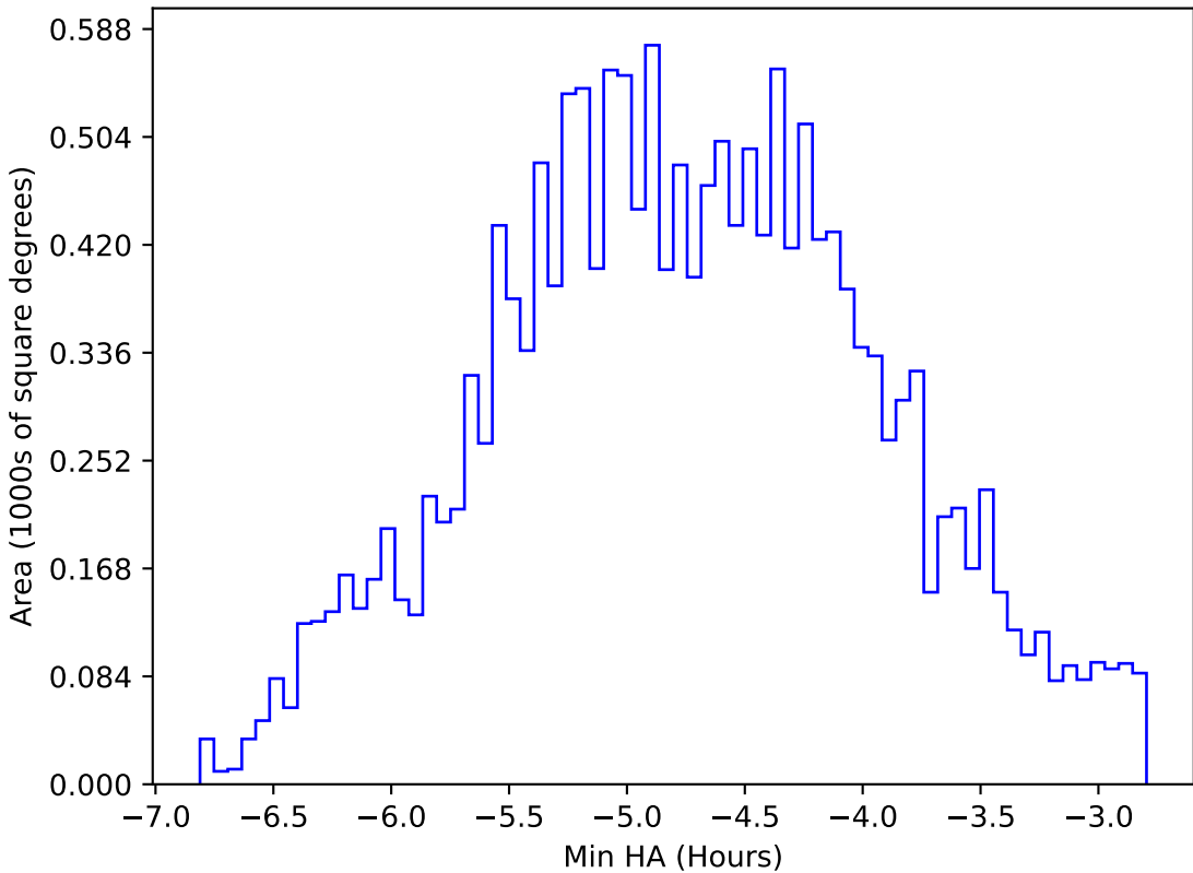
too_elab_r16_d3_giz_v3.4_10yrs WFD all bands: Min HA
