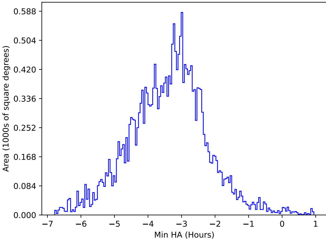
too_elab_r16_d3_giz_v3.4_10yrs All sky y band: Min HA
