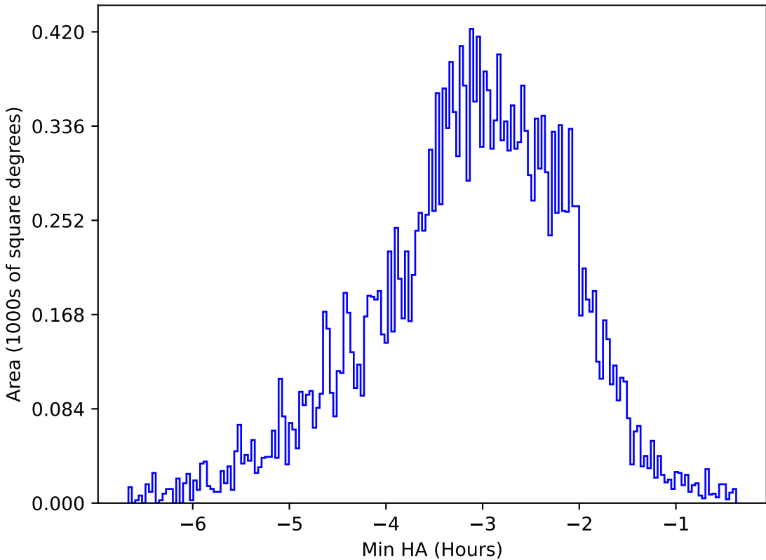
too_elab_r16_d3_giz_v3.4_10yrs All sky u band: Min HA
