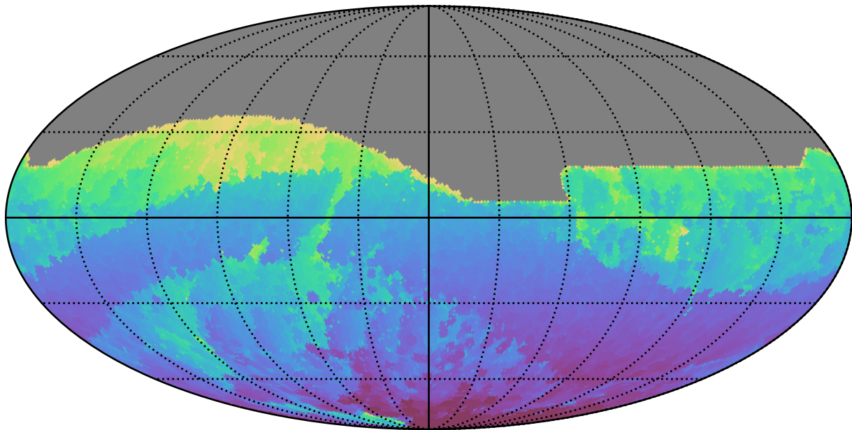
too_elab_r16_d3_giz_v3.4_10yrs All sky r band: Min HA
