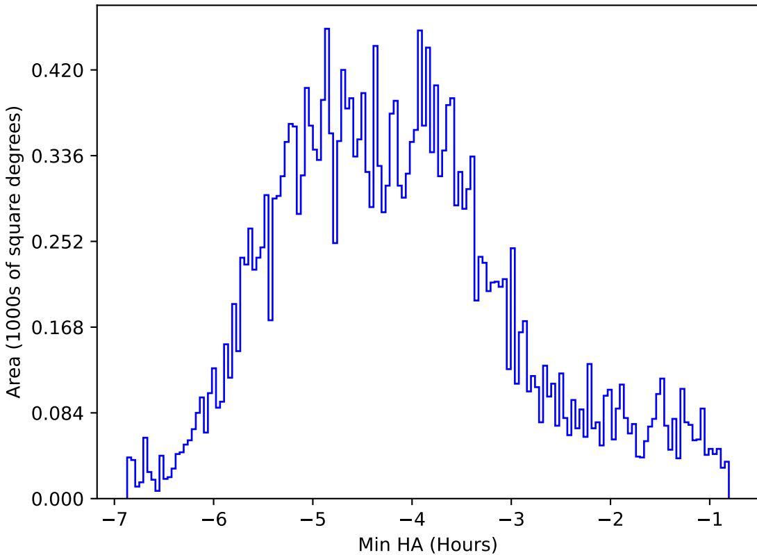
too_elab_r16_d3_giz_v3.4_10yrs All sky r band: Min HA
