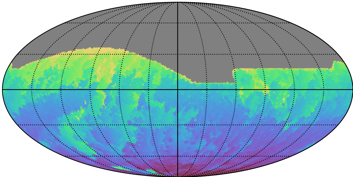
too_elab_r16_d3_giz_v3.4_10yrs All sky i band: Min HA
