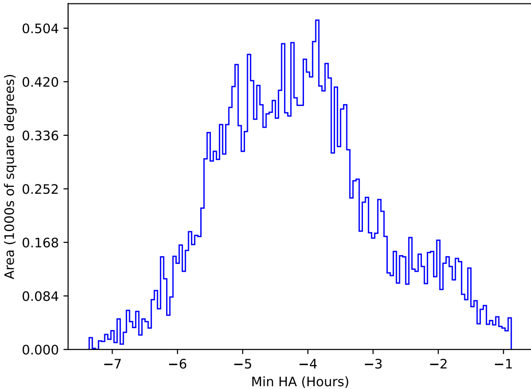
too_elab_r16_d3_giz_v3.4_10yrs All sky i band: Min HA
