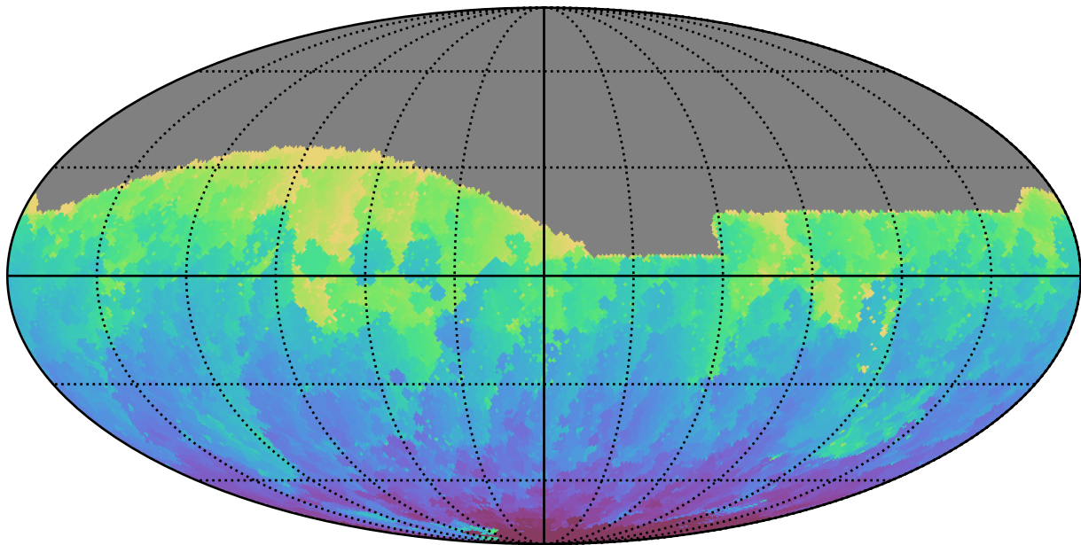
too_elab_r16_d3_giz_v3.4_10yrs All sky g band: Min HA
