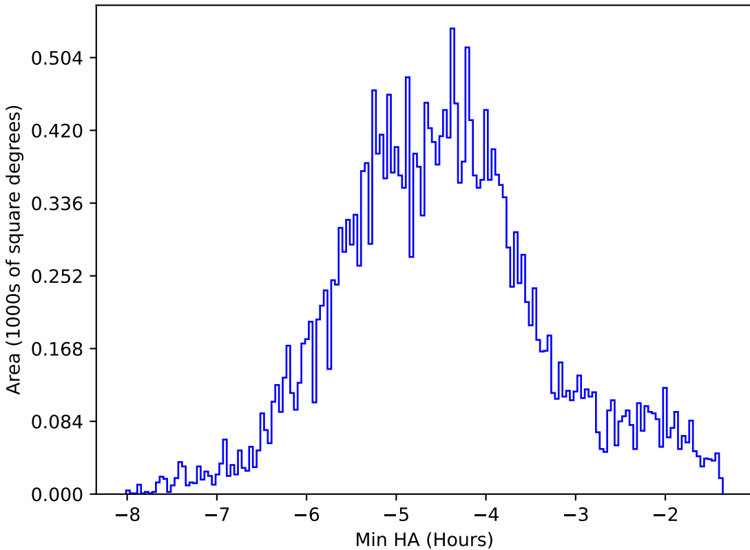
too_elab_r16_d3_giz_v3.4_10yrs All sky all bands: Min HA
