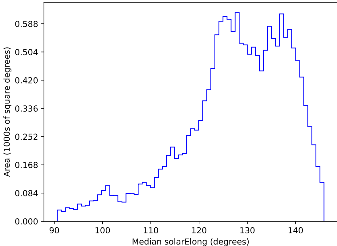
too_elab_r16_d3_giz_v3.4_10yrs WFD z band: Median solarElong
