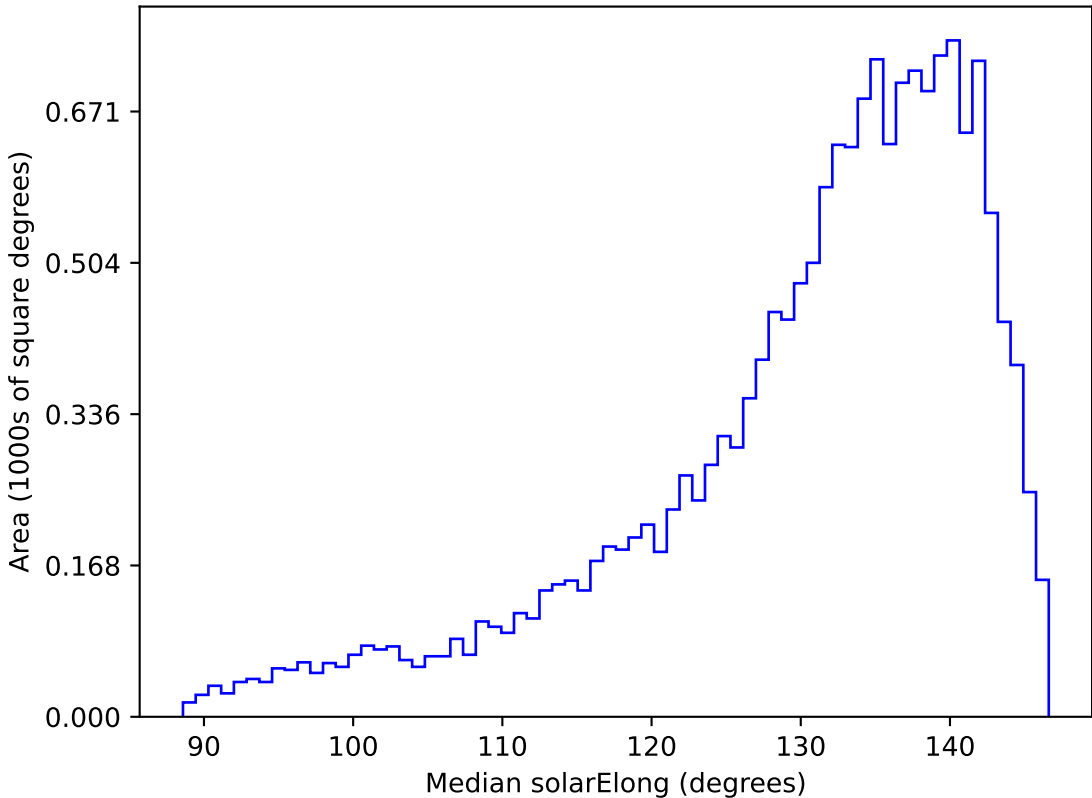
too_elab_r16_d3_giz_v3.4_10yrs WFD y band: Median solarElong
