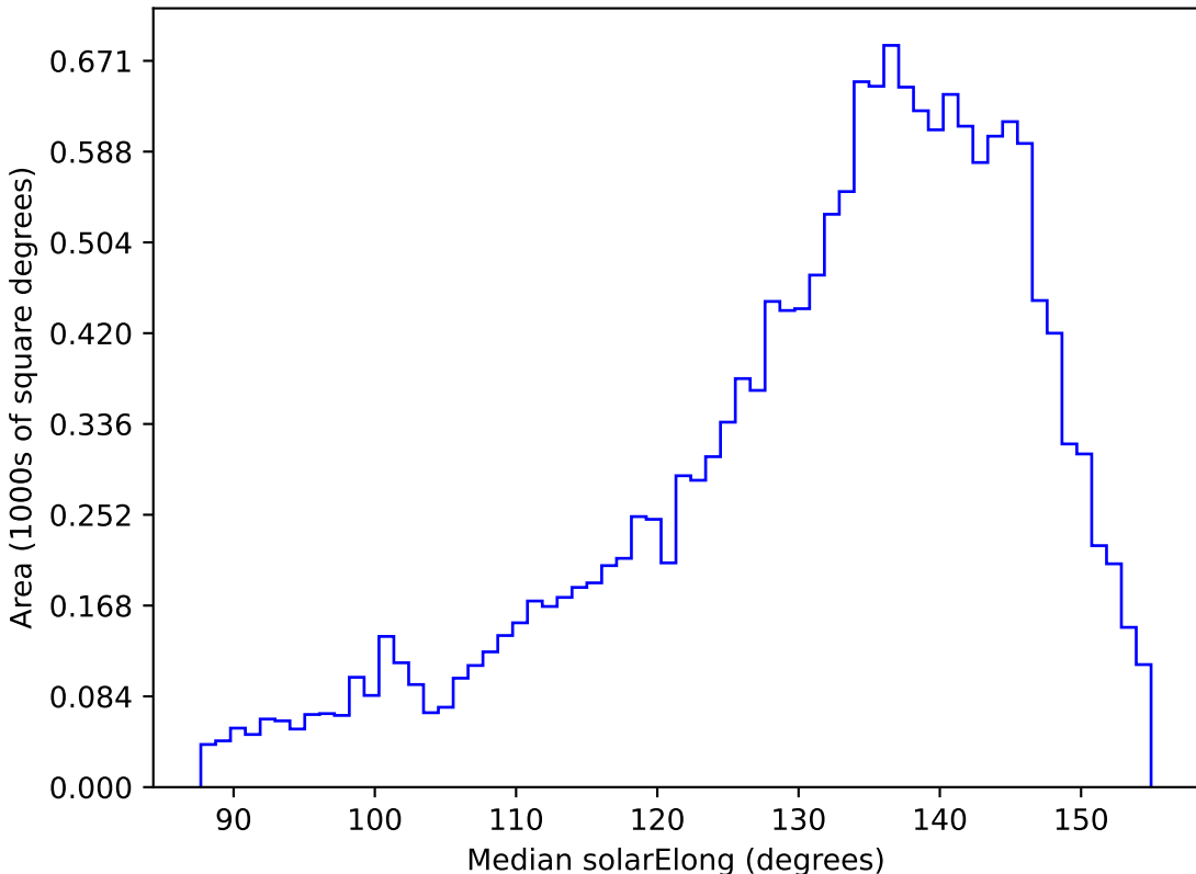
too_elab_r16_d3_giz_v3.4_10yrs WFD u band: Median solarElong
