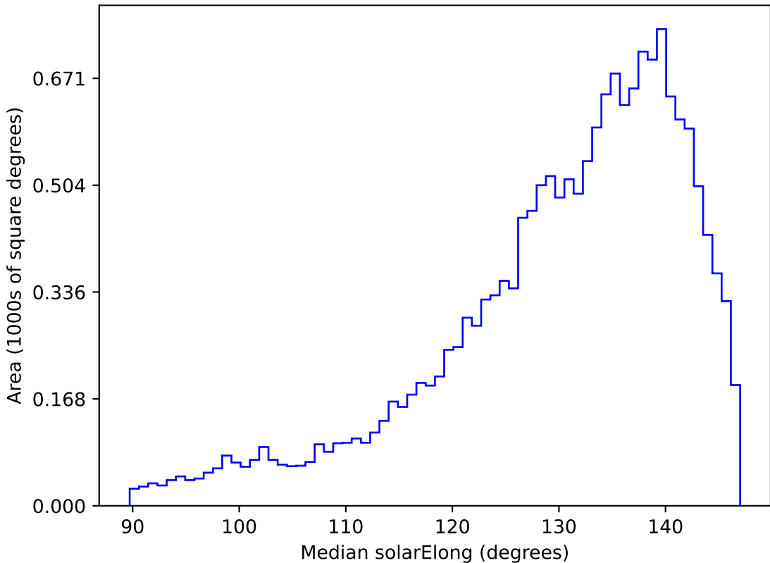
too_elab_r16_d3_giz_v3.4_10yrs WFD r band: Median solarElong
