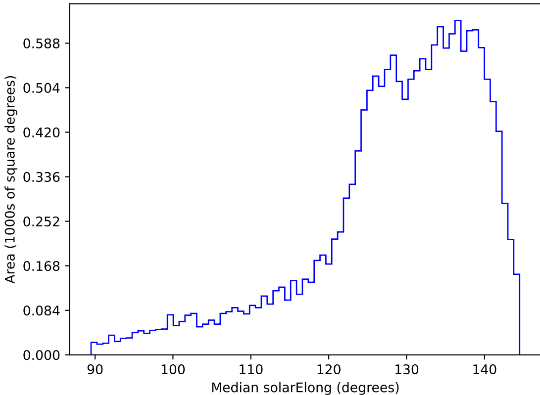
too_elab_r16_d3_giz_v3.4_10yrs WFD i band: Median solarElong
