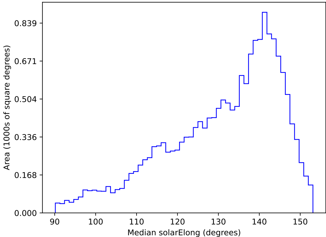
too_elab_r16_d3_giz_v3.4_10yrs WFD g band: Median solarElong
