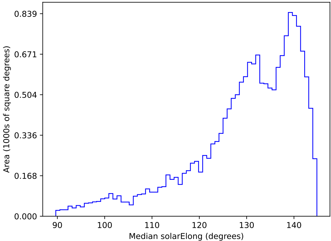
too_elab_r16_d3_giz_v3.4_10yrs WFD all bands: Median solarElong
