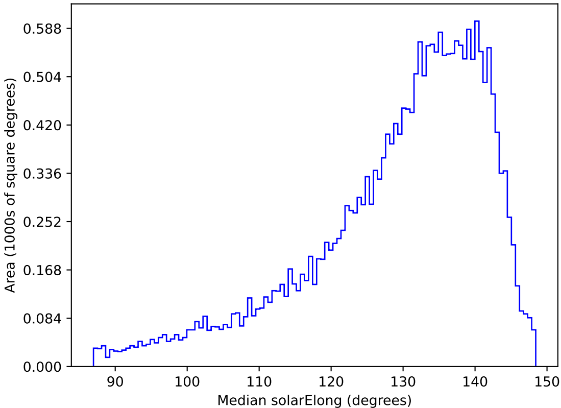
too_elab_r16_d3_giz_v3.4_10yrs All sky y band: Median solarElong
