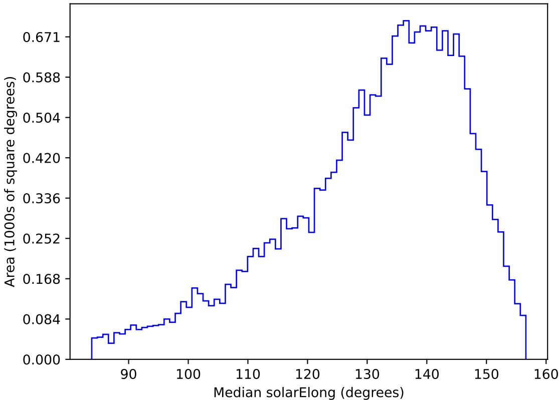
too_elab_r16_d3_giz_v3.4_10yrs All sky u band: Median solarElong
