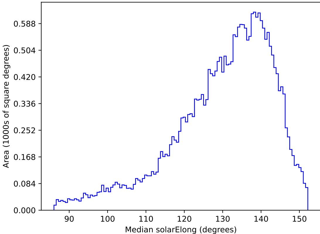
too_elab_r16_d3_giz_v3.4_10yrs All sky r band: Median solarElong
