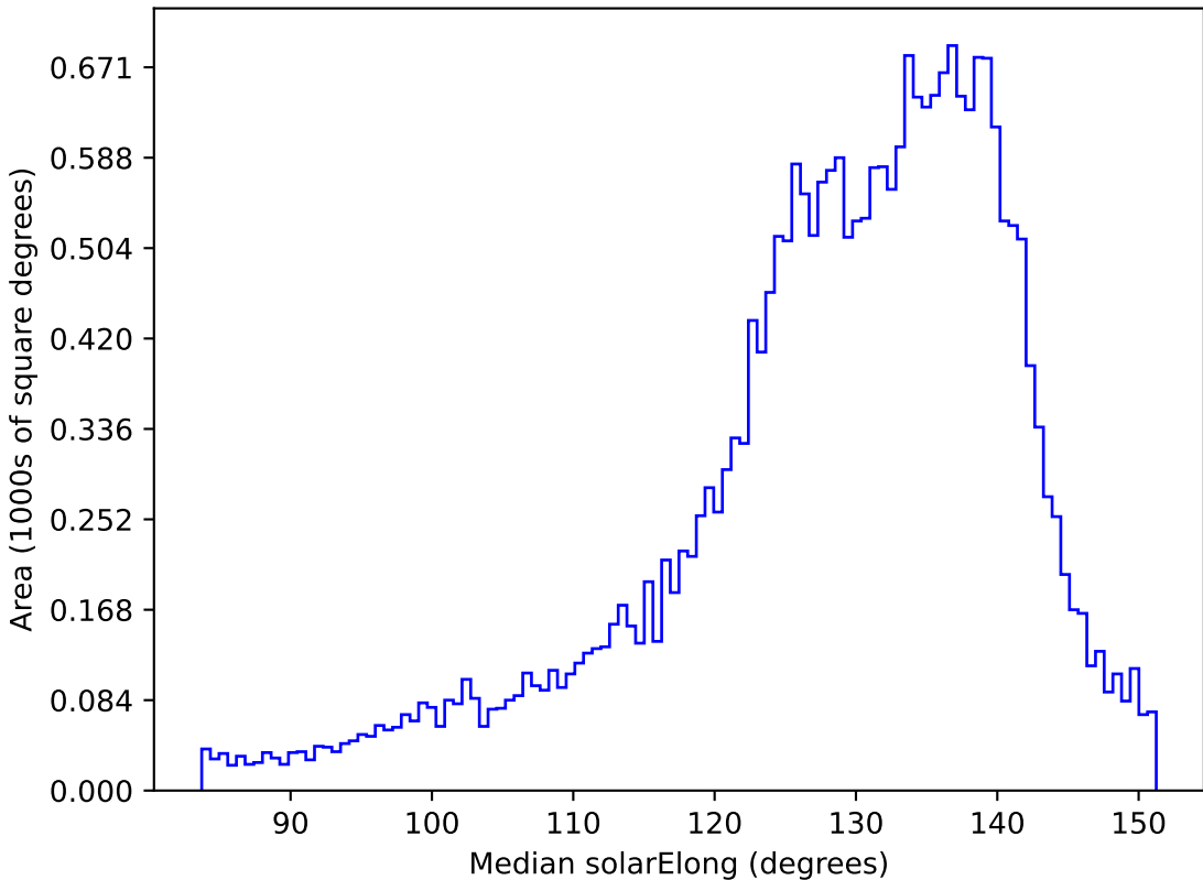
too_elab_r16_d3_giz_v3.4_10yrs All sky i band: Median solarElong
