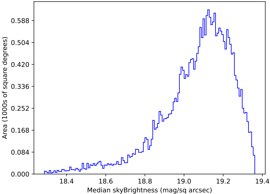
too_elab_r16_d3_giz_v3.4_10yrs Yr 1 z band: Median skyBrightness
