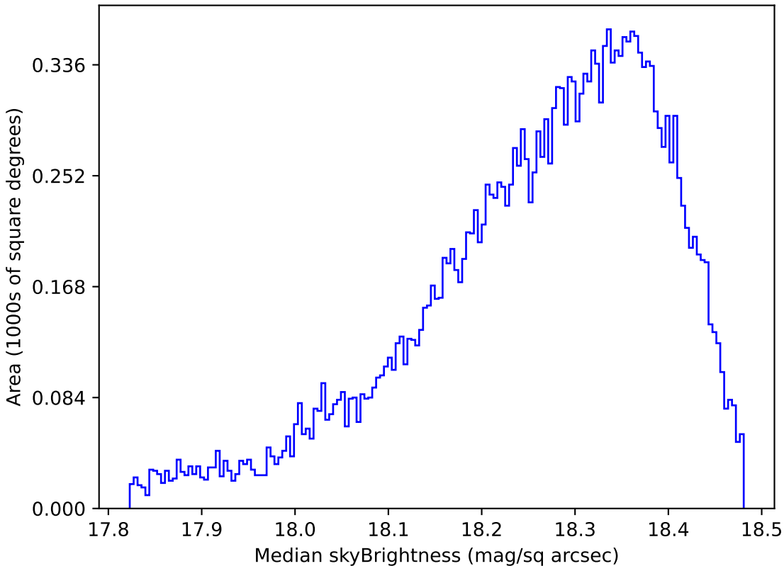
too_elab_r16_d3_giz_v3.4_10yrs Yr 1 y band: Median skyBrightness
