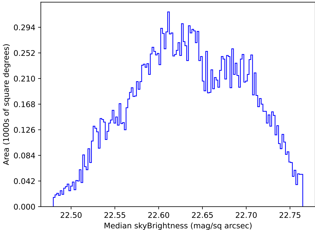
too_elab_r16_d3_giz_v3.4_10yrs Yr 1 u band: Median skyBrightness
