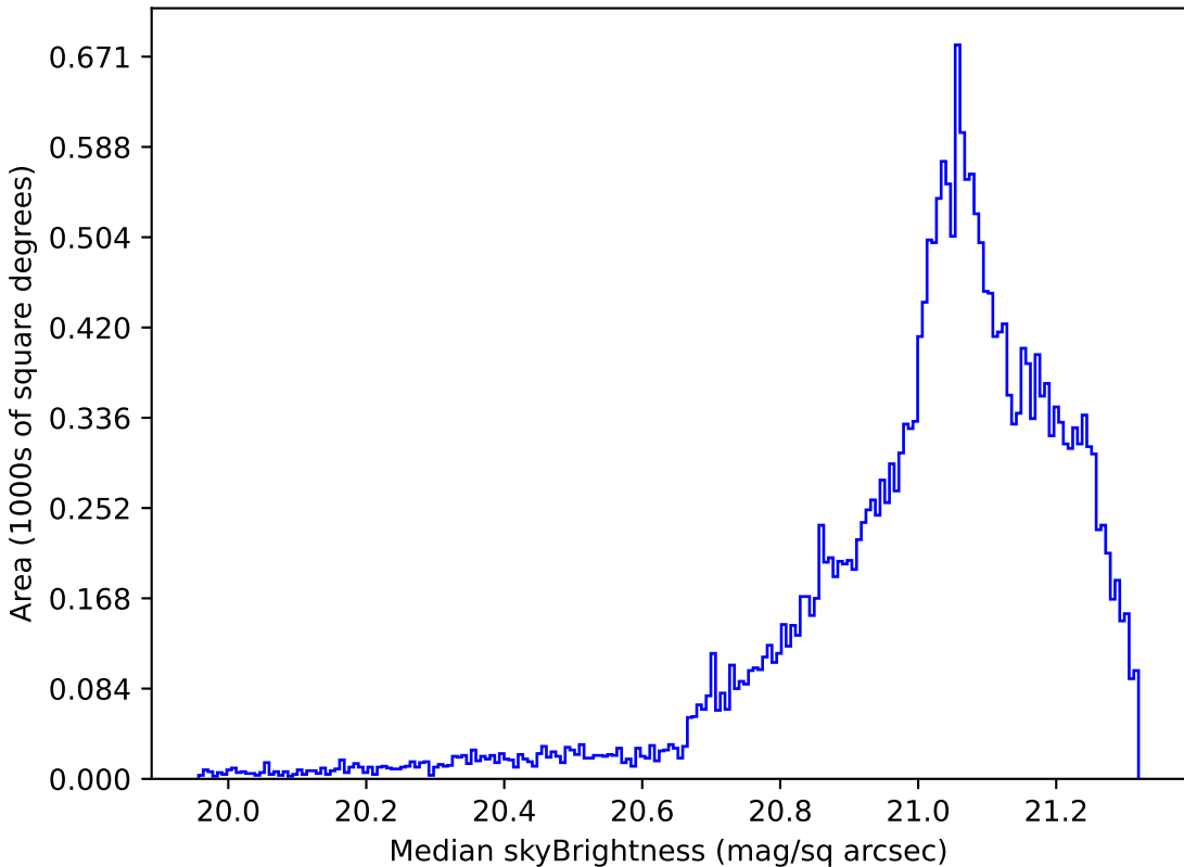
too_elab_r16_d3_giz_v3.4_10yrs Yr 1 r band: Median skyBrightness
