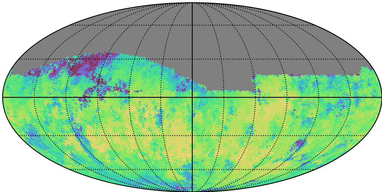
too_elab_r16_d3_giz_v3.4_10yrs Yr 1 i band: Median skyBrightness
