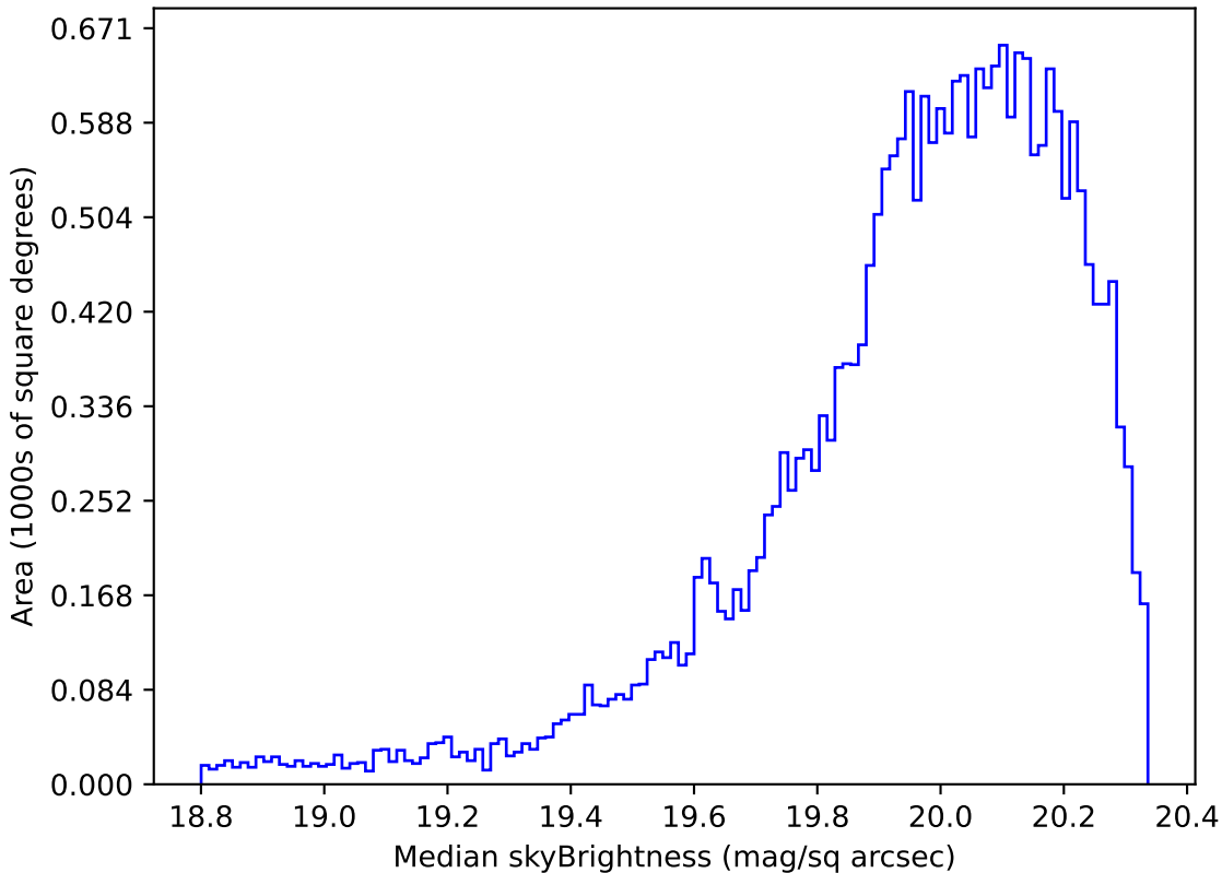
too_elab_r16_d3_giz_v3.4_10yrs Yr 1 i band: Median skyBrightness
